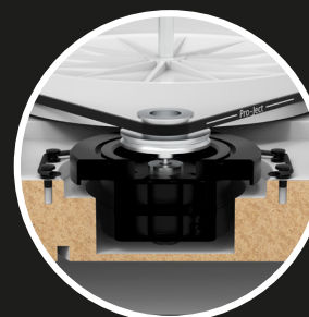
Superb motor suspension: no points of contact
