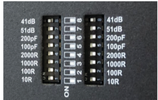
dip-switches
